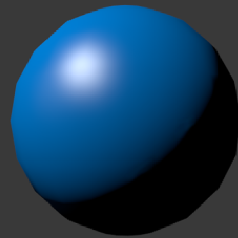
PHONG SHADING
