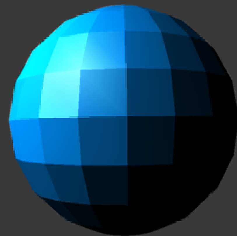
FLAT SHADING
